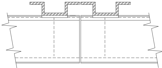
TYPICAL HORIZONTAL SECTION (HAT SUPPORTED)
