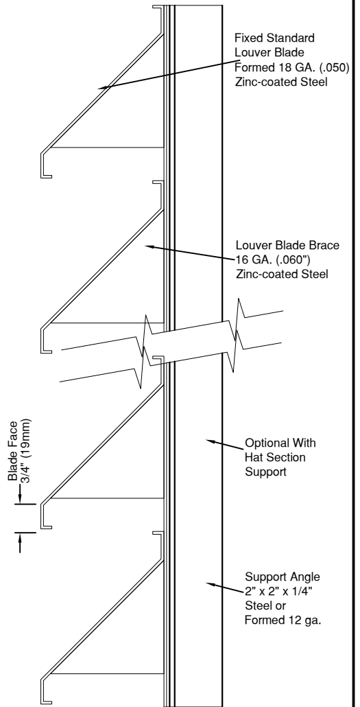
TYPICAL VERTICAL SECTION
