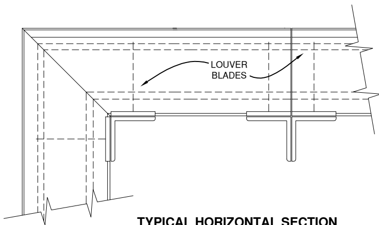
TYPICAL HORIZONTAL SECTION (MITERED CORNER)
