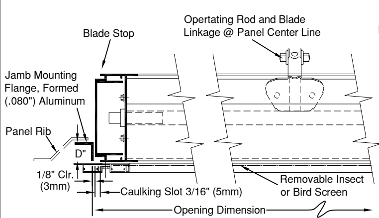
TYPICAL JAMB
