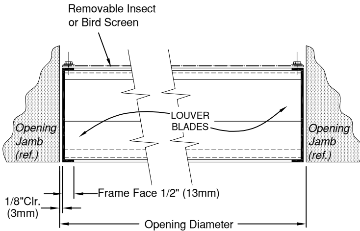
TYPICAL HORIZONTAL SECTION
