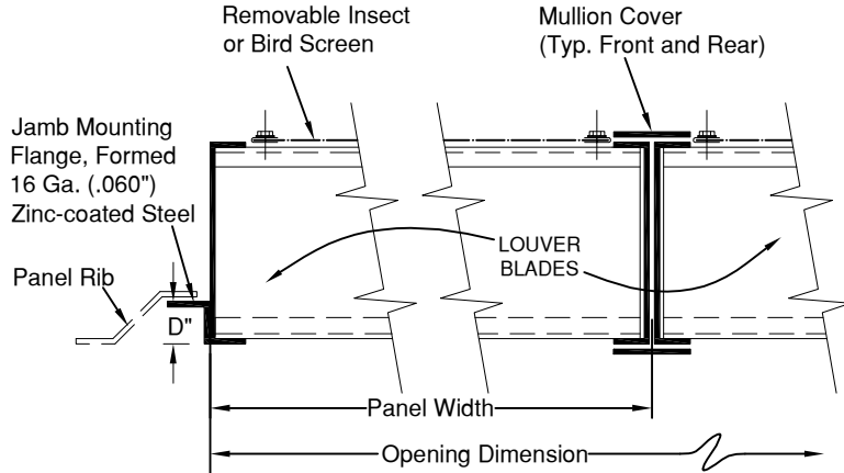
TYPICAL HORIZONTAL SECTION
