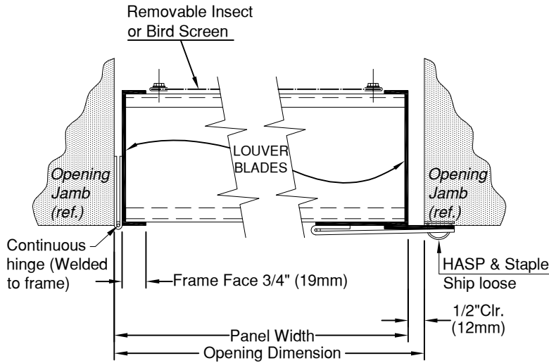
TYPICAL HORIZONTAL SECTION
